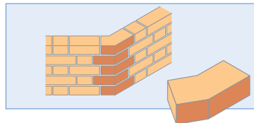
BD.1.3 Standard Brick Fair Faced on Bed Surface
