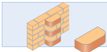
BN.2.1/BN.2.2 Double Bullnose
